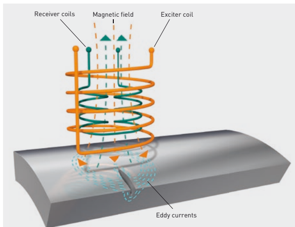
The principle behind eddy current testing
